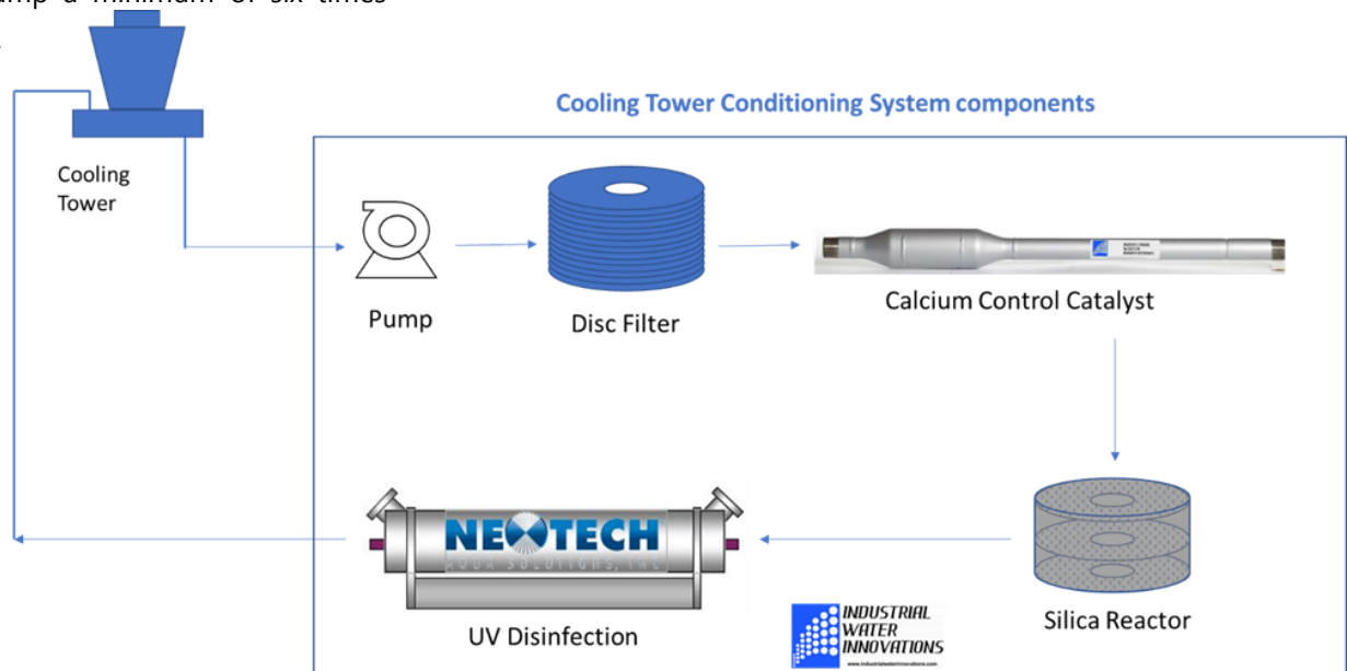
Figure 5 - Cooling Tower Conditioning System Schematic
